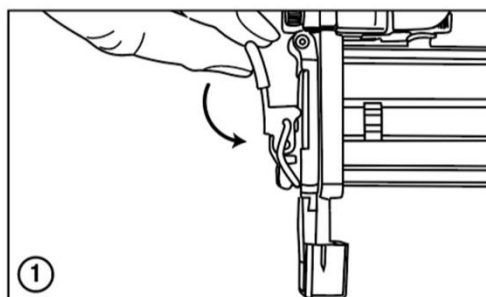
Fig. F – Removing a jammed fastener
